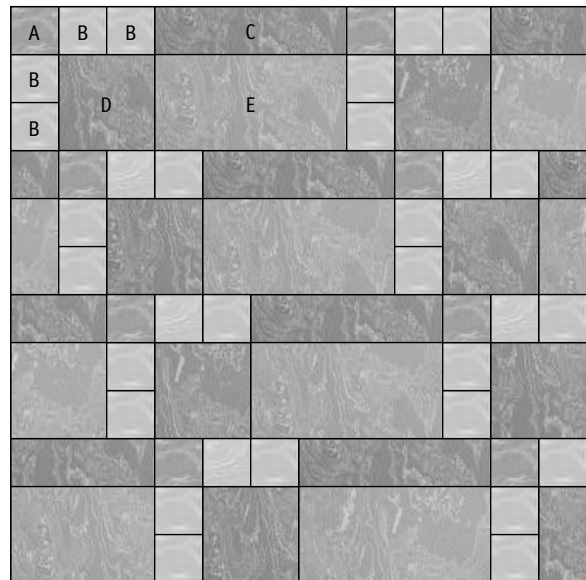
Mesto Configurations Floor Design #104
